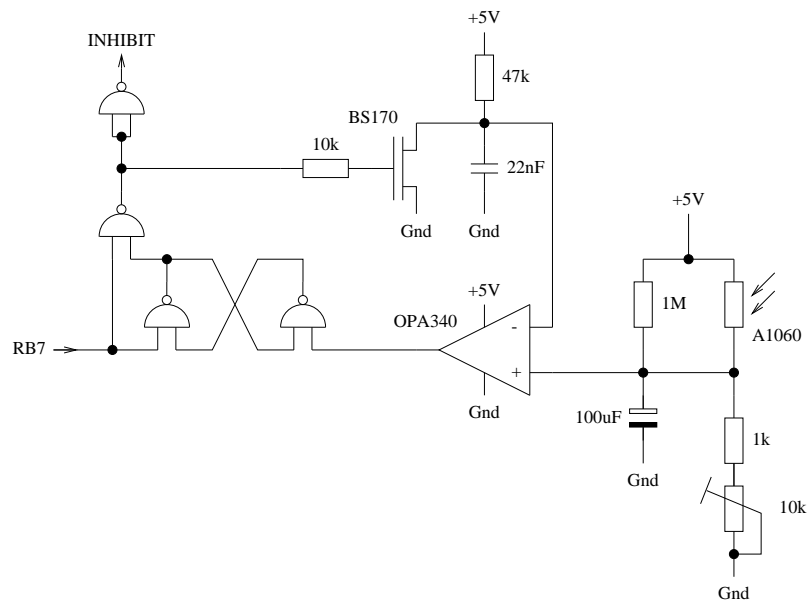
Figure 4: Circuit Diagram of Brightness Control
