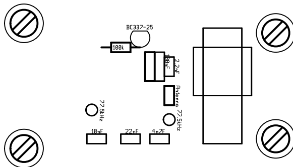
Figure 8: Printed Circuit Board of Receiver (Silk)
