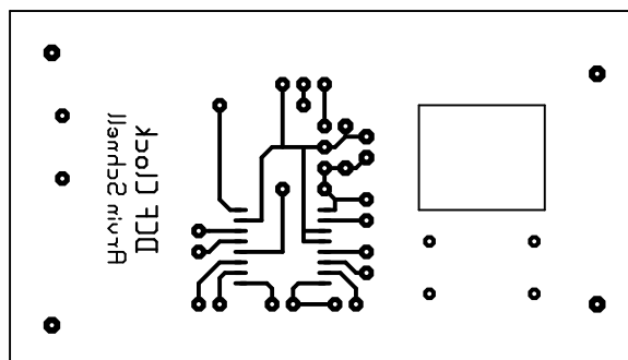
Figure 10: Printed Circuit Board of Receiver (Solder)
