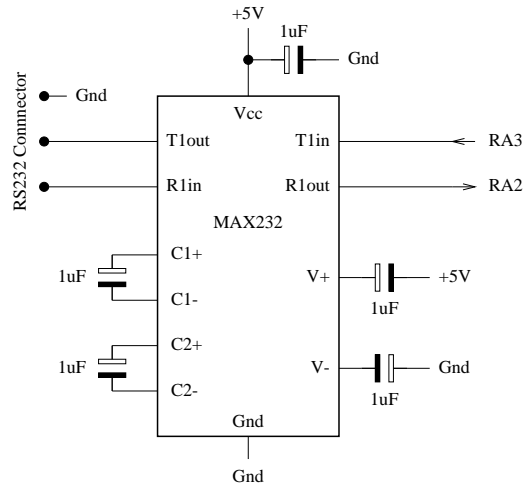
Figure 5: Circuit Diagram of RS232 Interface
