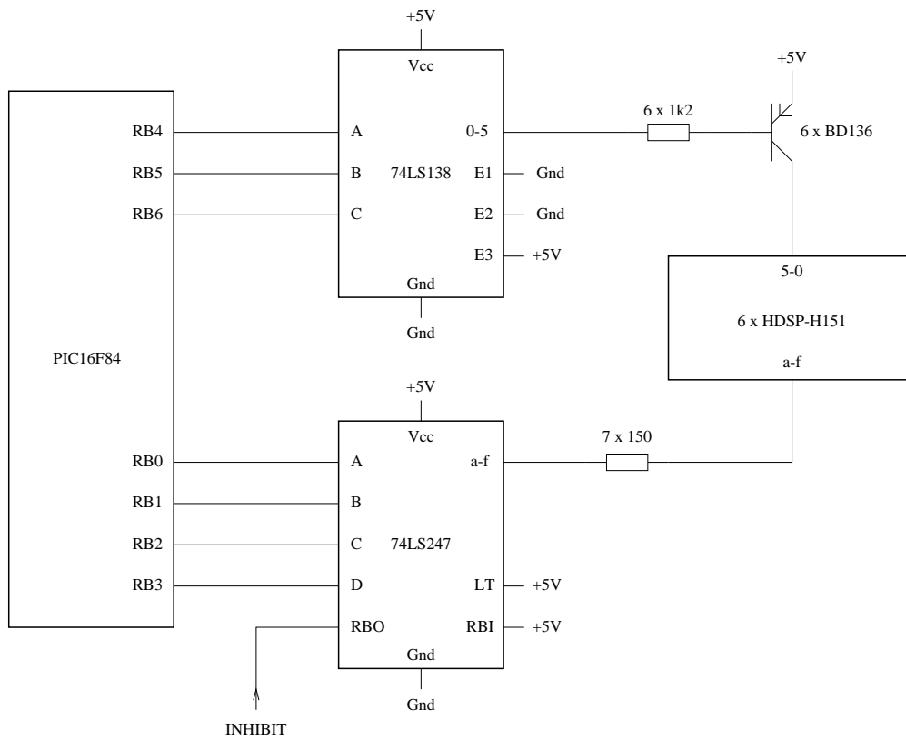
Figure 3: Circuit Diagram of Display Stuff
