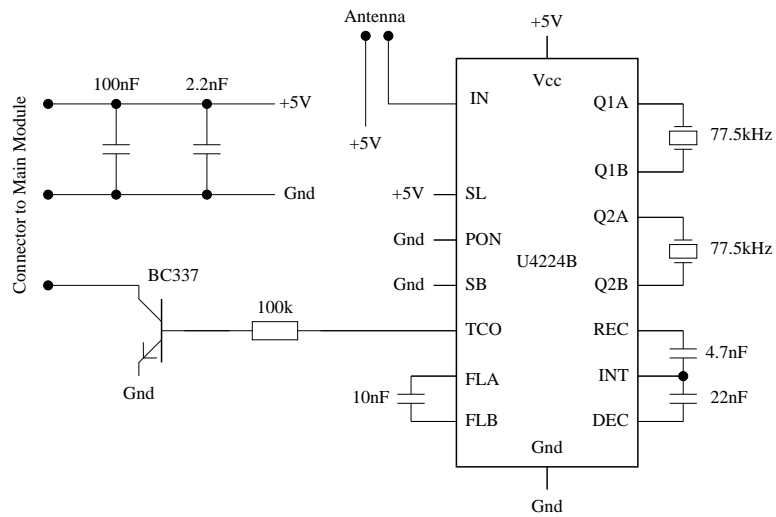
Figure 6: Circuit Diagram of Receiver
