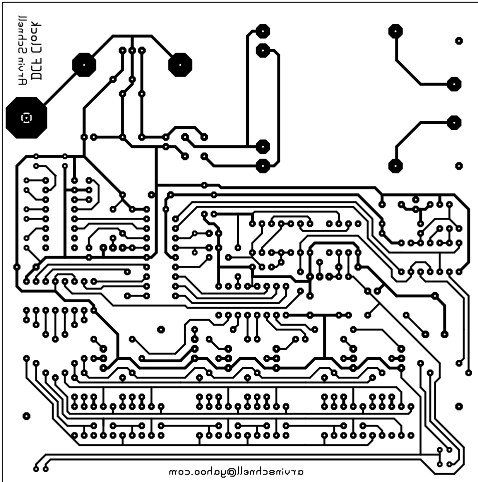
Figure 9: Printed Circuit Board of Main Module (Solder)
