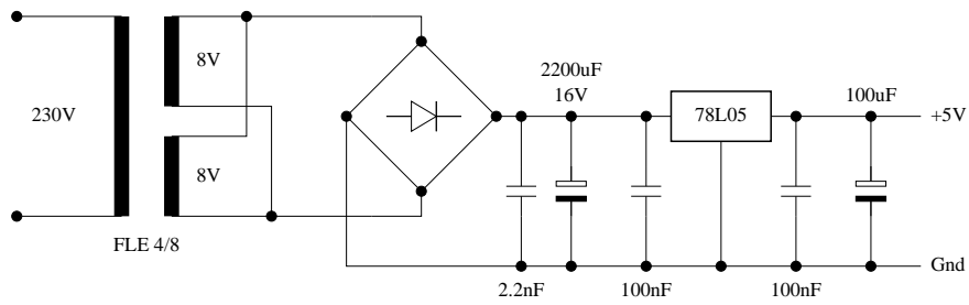
Figure 2: Circuit Diagram of Power Supply
