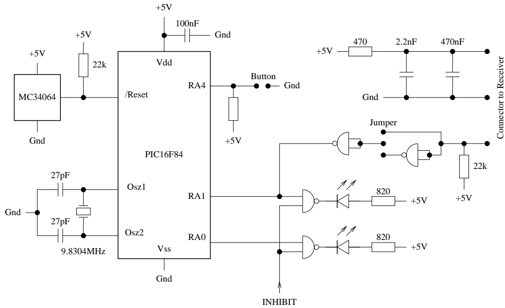
Figure 1: Circuit Diagram of Main Stuff
