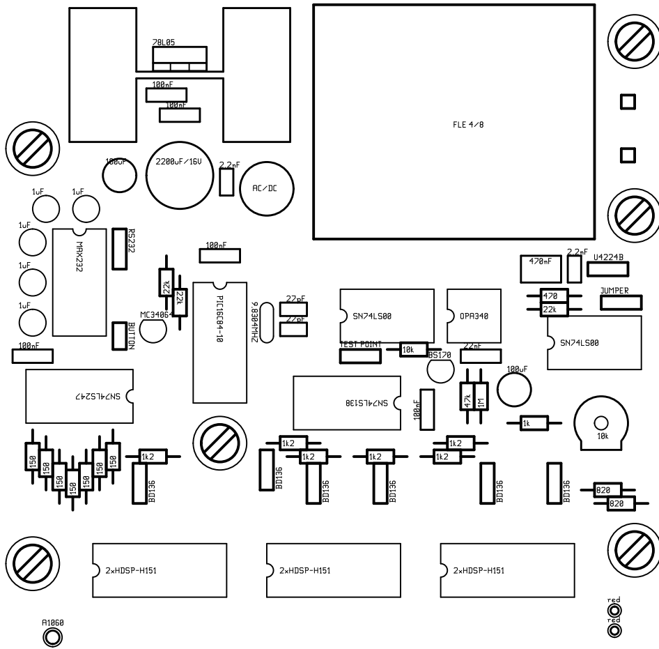
Figure 7: Printed Circuit Board of Main Module (Silk)
